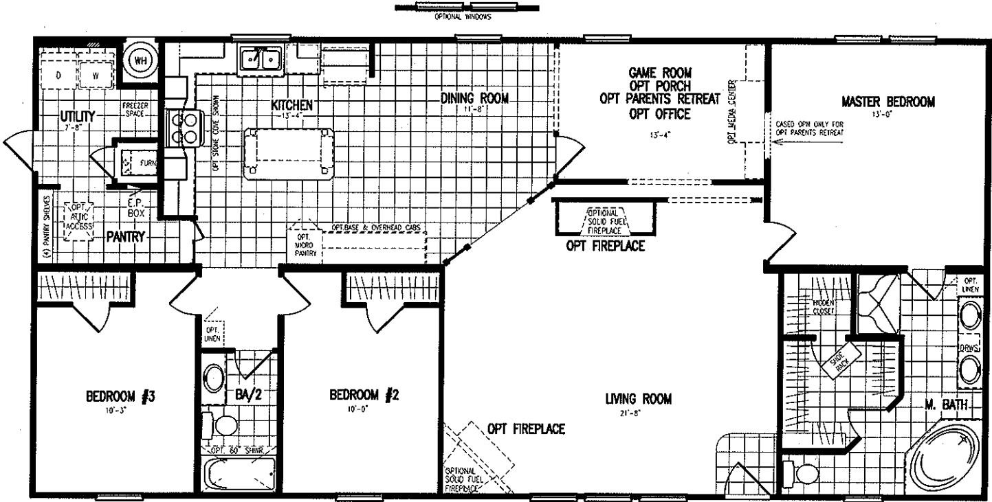
MODEL PI-4061 30' x 62' BOX 1860 SQ. FT.. 3 BEDROOMS, 2 BATHS OPTIONAL POPCI
