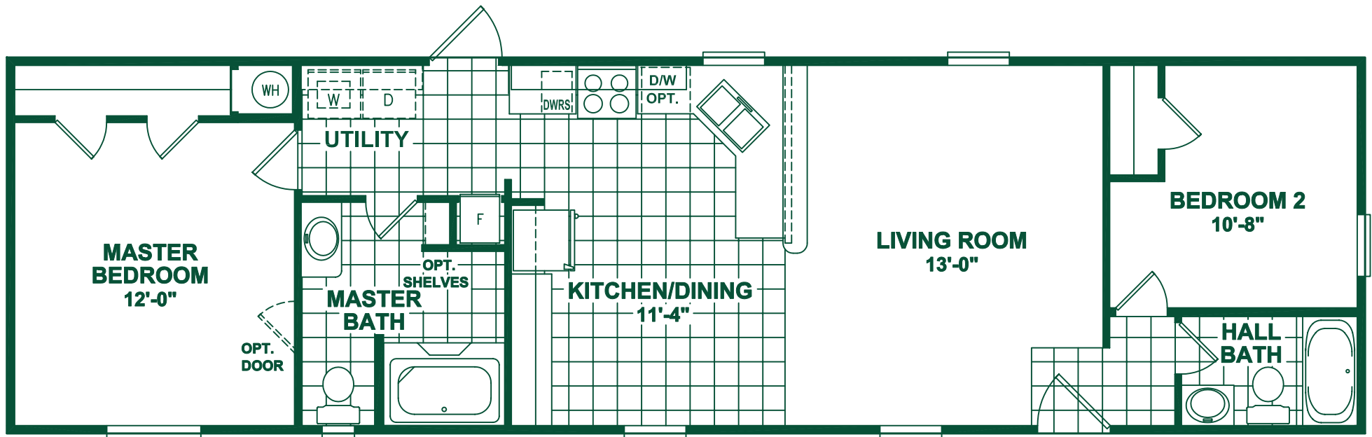
MODEL: 302 16'x56' (60' OVERALL) APPROX. 868 SQ. FT. 2 BEDROOM, 2 BATH
