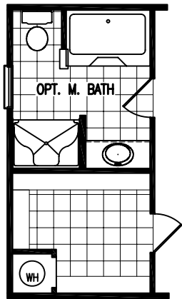
MODEL SS-9003 18' x 76' 1330 SQ. FT.. 3 BEDROOMS, 2 BATHS
