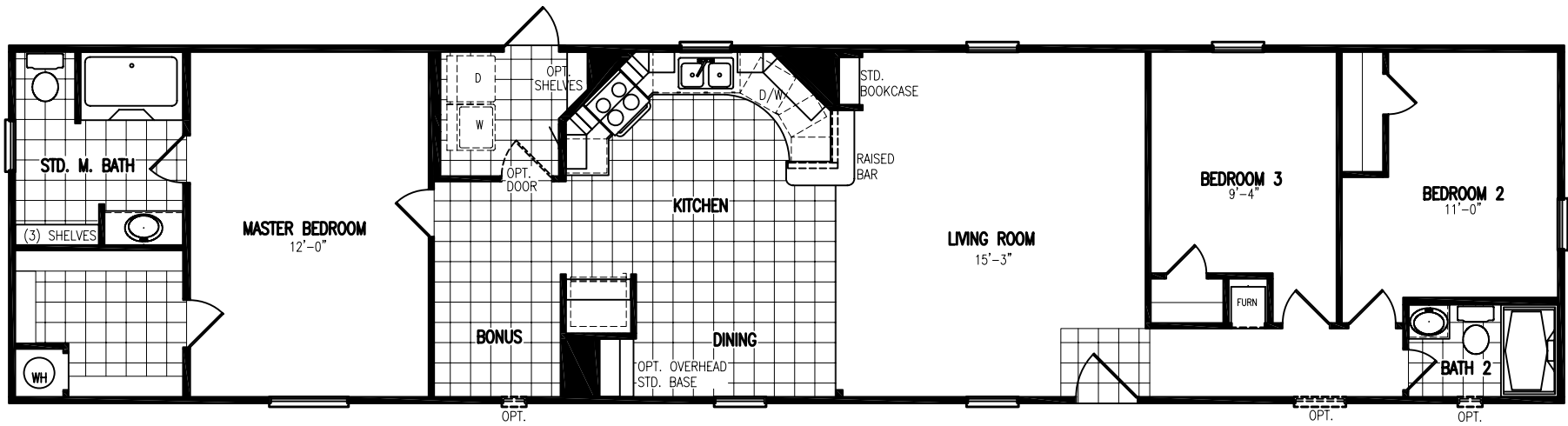
MODEL SS-9003 18' x 76' 1330 SQ. FT.. 3 BEDROOMS, 2 BATHS
