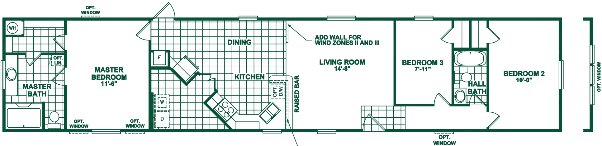
MODEL: 381 16'x76' (80' OVERALL) APPROX. 1178 SQ. FT. 3 BEDROOM, 2 BATH
