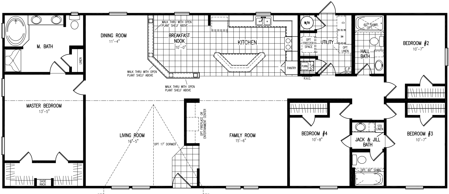
MODEL: PI-4006 30'-0" X 76'-0" 2280 SQ. FT. (BOX SIZE) 4 BEDROOMS, 3 BATHS
