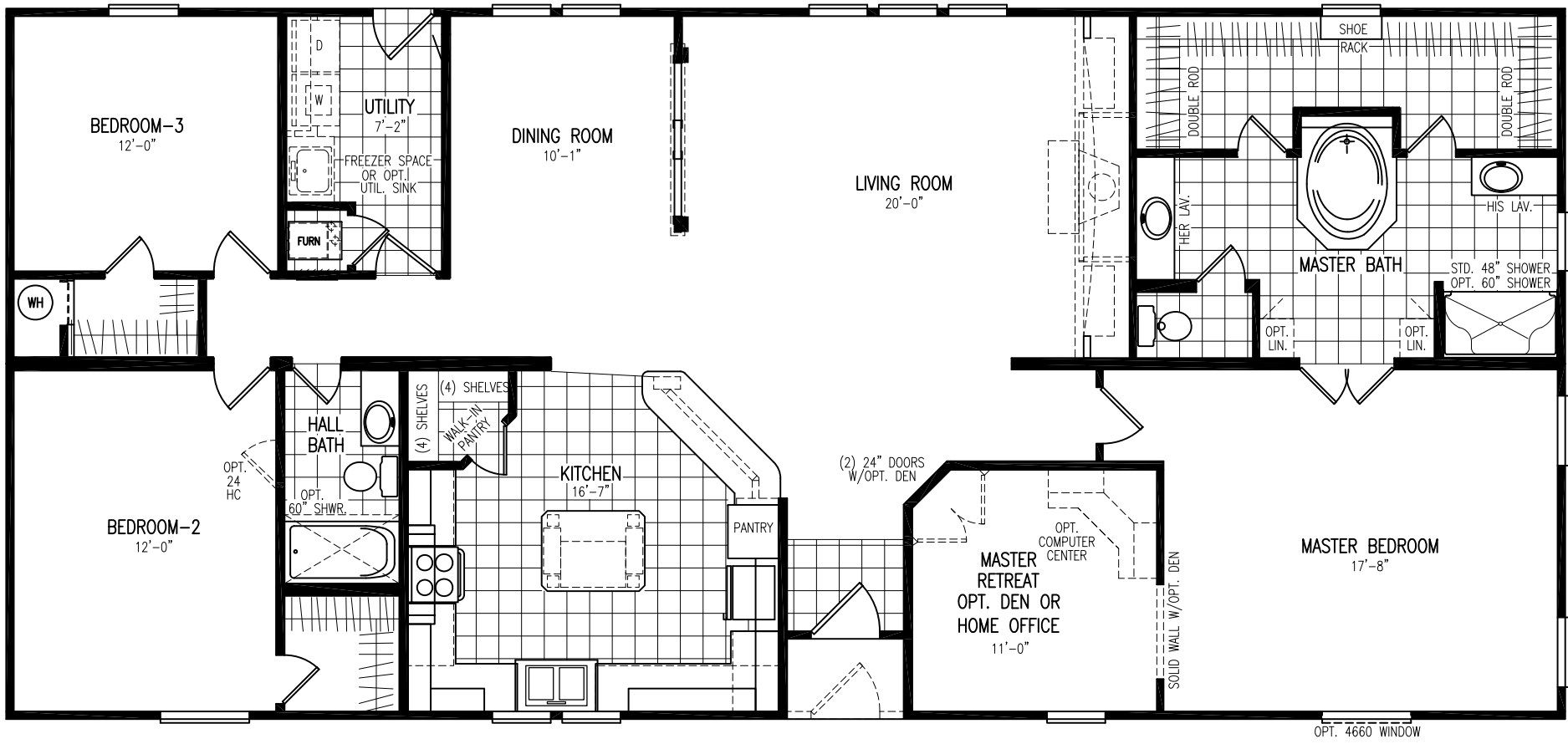
MODEL: PI-4204 31' x 68' BOX SIZE (2108 SQ. FT.) 3 BEDROOMS, 2 BATHS
